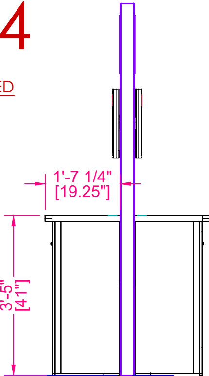
SIDE VIEW Scale - 1/2" = 1'
