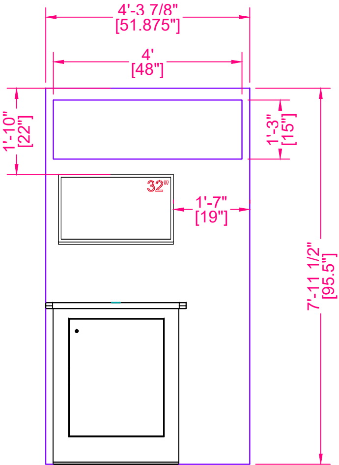
FRONT VIEW Scale - 1/2" = 1'
