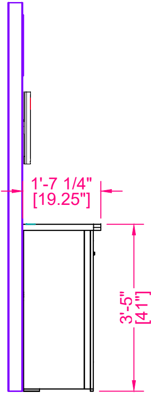
SIDE VIEW Scale - 1/2" = 1'
